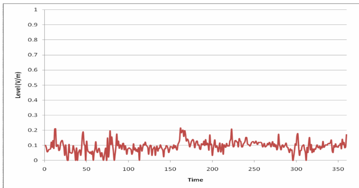
Electric field strengths recorded over 6 min period using 3 GHz probe at point of max NIR:
